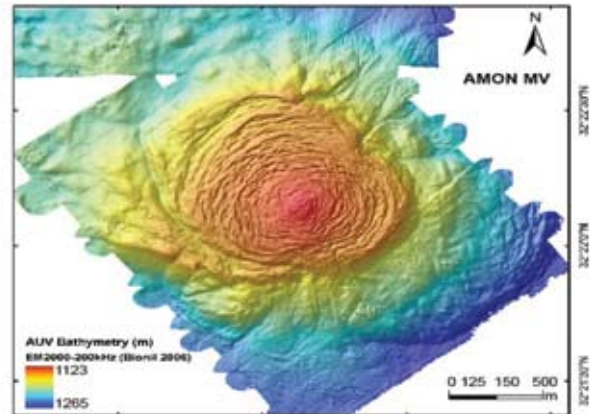
Figure 28. The Amon mud volcano in the Nile Cone, offshore Egypt, Dupre, et. al., 2008
