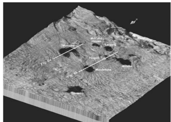
Figure 32. Mud Volcanoes offshore Southern Crete. Backscatter data 7 superimposed on 3D seafloor relief view of the Eastern Olimpi field. Huguen et al., 2004, Marine Geology 209: 245-263
