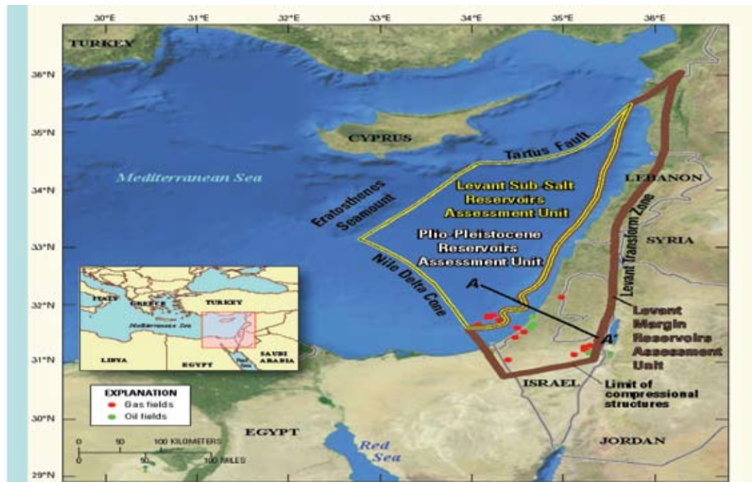
Figure 7. The Levantine Basin with its recent oil and gas discoveries. Assessed potential for further discoveries of natural gas 122 tcf and oil 1,7 billion barrels, USGS Technical Report, 2010
