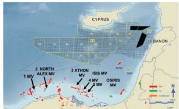
Figure 30. Location of Active Mud Flow Volcanoes (MV) in relation to the natural gas deposits in the Nile Cone, offshore Egypt. Figures 27 and 29 combined.
