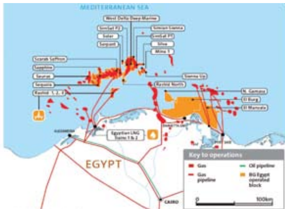
Figure 29. Distribution of natural gas reservoirs offshore Egypt, Neftegaz, EU, 2010 Rigzone, 2010
