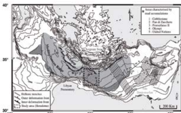
Figure 31. Morphostructural sketch of the Mediterranean Ridge (MR) (modified from Chaumillon et al., 1996; Robertson and Shipboard Scientific Party, 1996; Cronin et al., 1997). Locations of the Prisms 2 (February 1998) track map and of the study area are indicated. Huguen et. al., 2004 Marine Geology
