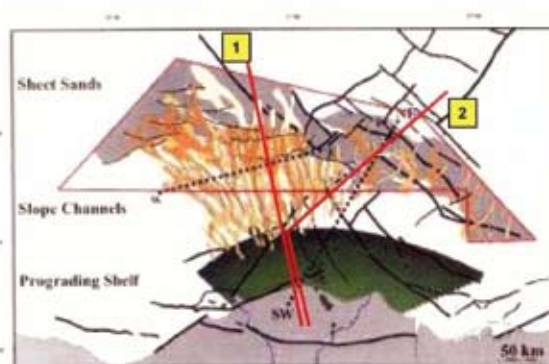
Figure 19a: Pliocene turbiditic system deposition
