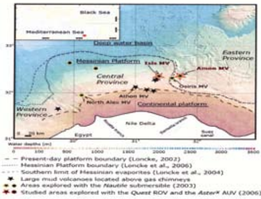
Figure 27. Active Mud Volcanoes in the Nile Cone, Dupre, et. al., 2008
