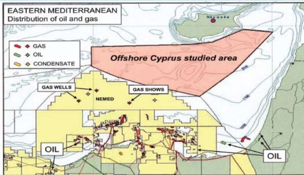
Figure 13. Distribution of oil and gas Fields and Discoveries in Eastern Mediterranean. Of interest are the 2 gas fields discovered by Shell, due to their proximity to the Greek and Cypriot Herodotus Basin. BEICIP/FRANLAB, 2007
