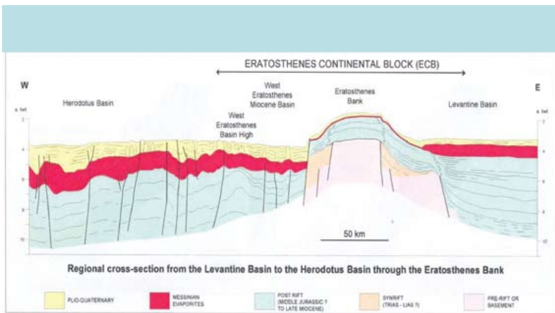
Figure 8. Regional cross – section from the Levantine basin to Herodotus Basin through the Eratosthenes Bank. Montadert and Nikolaides, 2007.
