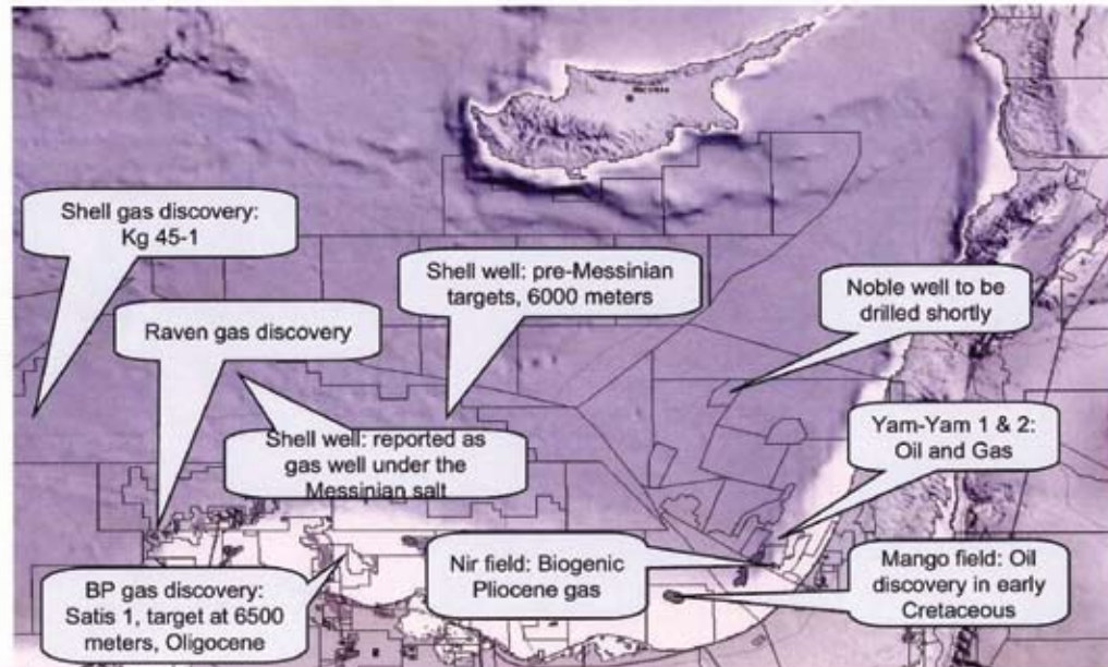
Figure 15. Hydrocarbon discoveries in the Nile Cone and Southern Levantine Basin, Kassinis, 2008
